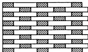
9 Flemish bond: 1 header, 1 stretcher; alternated each course
